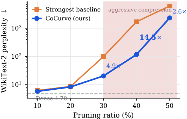
(a) Perplexity advantage widens with compression
