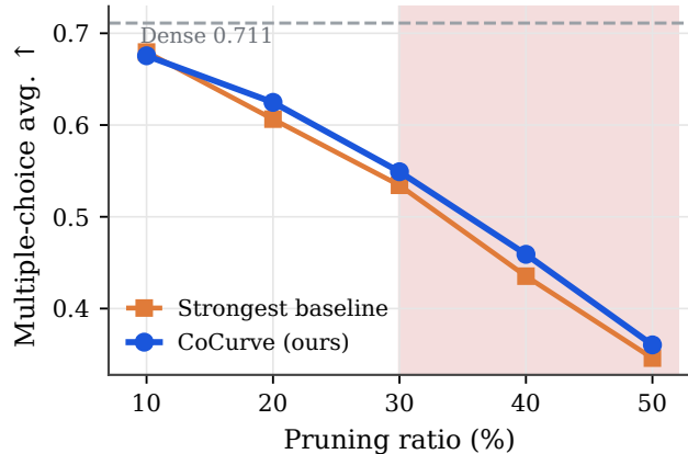
(b) Accuracy leads from 20% up
